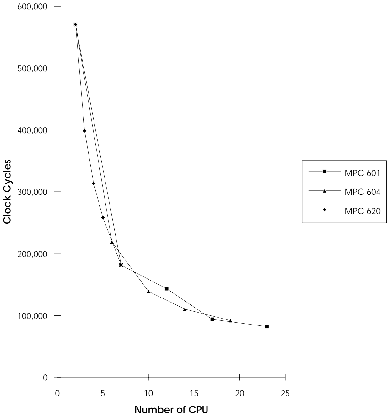
Total Clock Cycles for Completion of Parallel Program (Queen) vs. Number of CPUs
